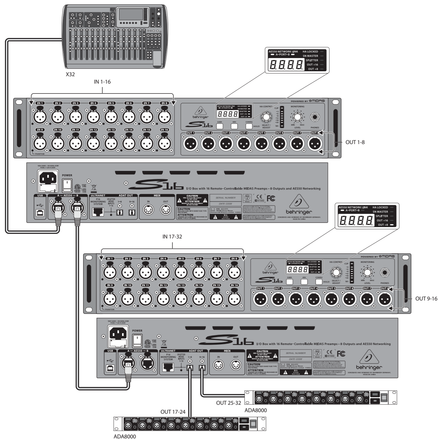
Linking two S16 units
